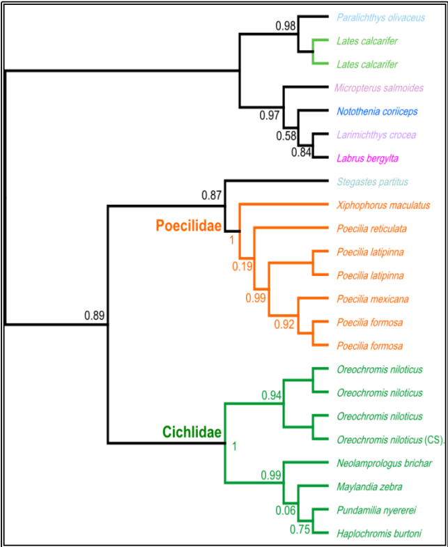
Fig. (2): Maximum likelihood phylogenetic tree based on the partial sequence of CYP450, where Cichlidae (green) and Poeciliidae (orange) families are well defined. Each other species were coloured according to its family assignment.
