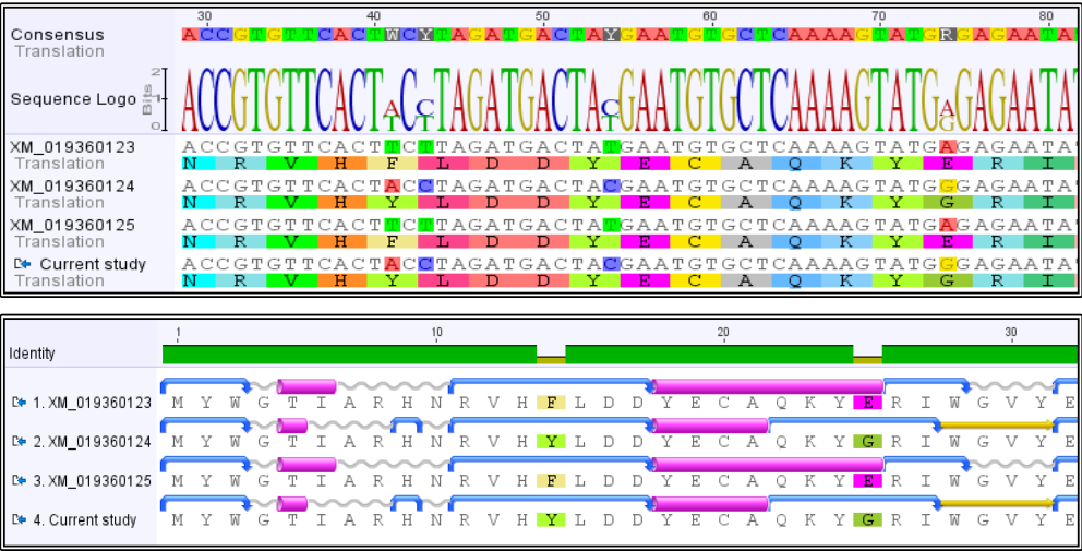
Fig. (1): Windows of 52 nucleotides of a pairwise alignment between O. niloticus CYP450 partial sequence. Four sites were polymorphic, while only two showed changes in amino acid sequence (Above). Prediction of protein secondary structure is indicated as: blue turns, grey coils, Pink alpha helix and yellow beta strands (below).
