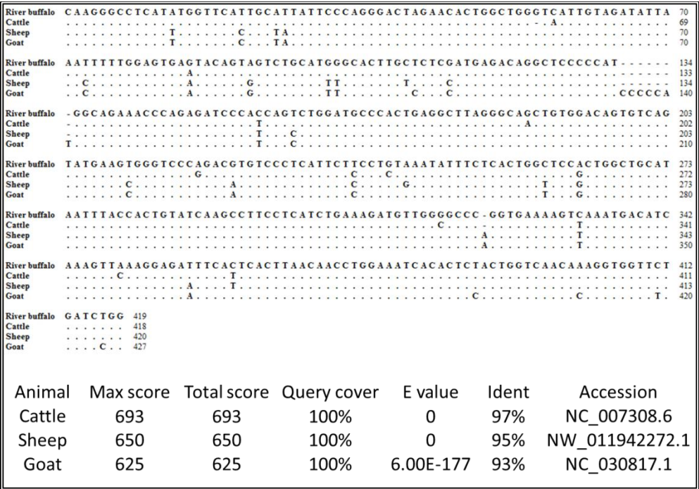
Fig. (3): The nucleotides sequence homology among the amplified region of CYP19 promoter in Egyptian river buffalo and some species.
