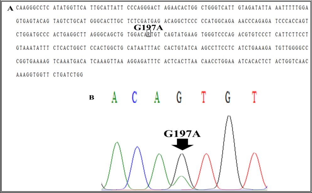
Fig. (2): The nucleotide sequence and the detected SNP in the Egyptian river buffalo CYP19 promoter amplified fragment.
