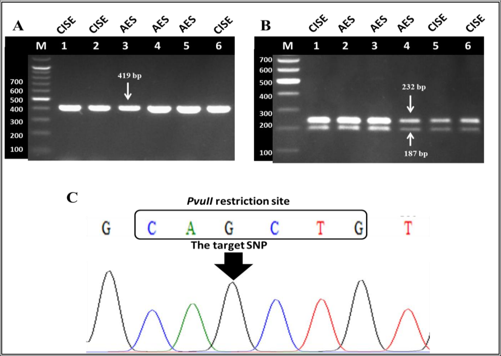
Fig. (1): The PCR product, PCR-RFLP pattern and sequencing result of the amplified CYP19-promotor fragment. A) The PCR product of CYP19 fragment. B) The PCR-RFLP pattern of the CYP19 gene amplicon. C) A part of CYP19 fragment sequencing chromatogram. CISE: Cattle Information System/Egypt. AES: Agricultural Experiments Station. M: 100 bp molecular marker.
